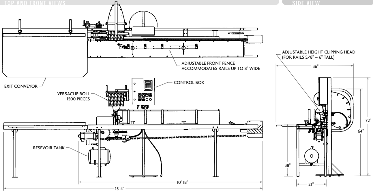
TOP AND FRONT VIEWS
